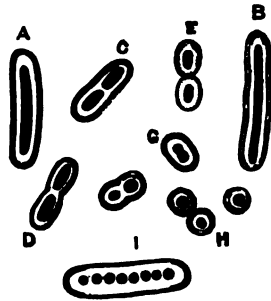
FIG. 68.—BACTERIUM PNEUMONIAE CROUPOSA, \times 1500 (after Zopf).
